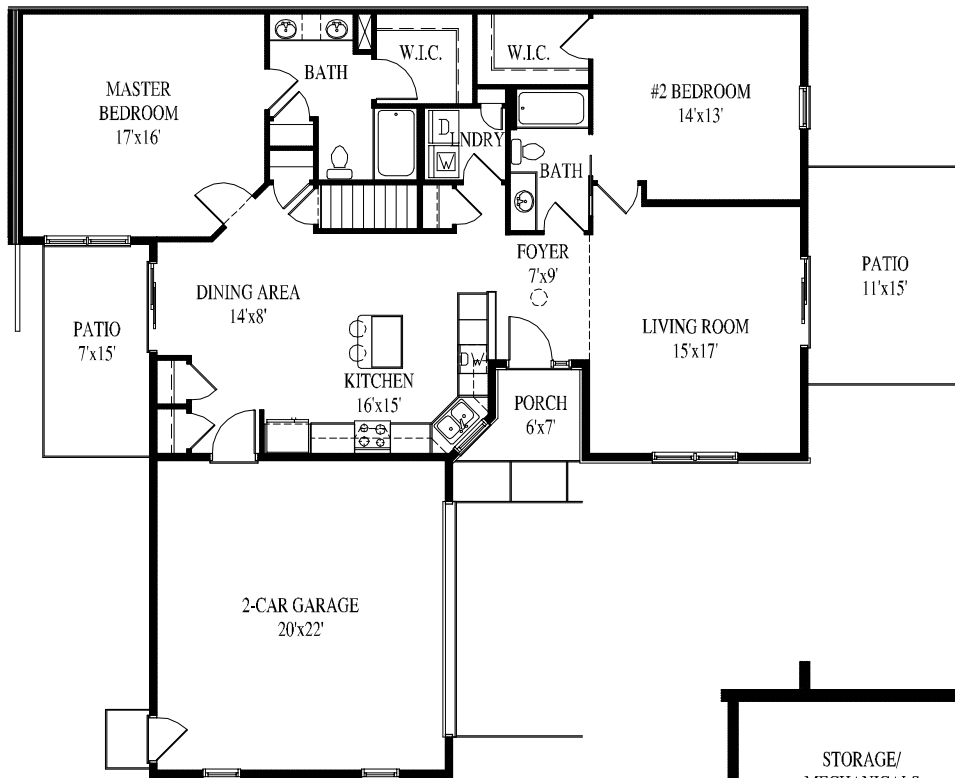
FLOOR PLAN 1549 SQ. FT.
