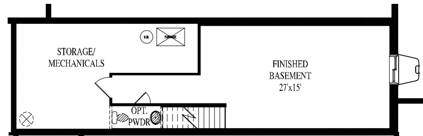
OPTIONAL FINISHED BASEMENT PLAN 460 SQ. FT.
